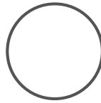
WAXING CRESCENT
