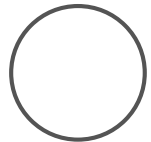
WANING GIBBOUS
