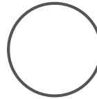
NEW MOON
