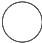
THIRD QUARTER
