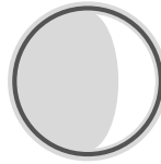
WAXING CRESCENT
