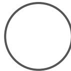
WANING CRESCENT
