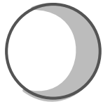
WANING GIBBOUS
