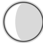
WANING CRESCENT
