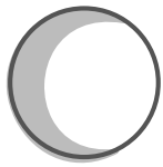
WAXING GIBBOUS
